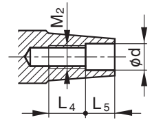
Pulley interface
