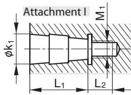
Tool interface
